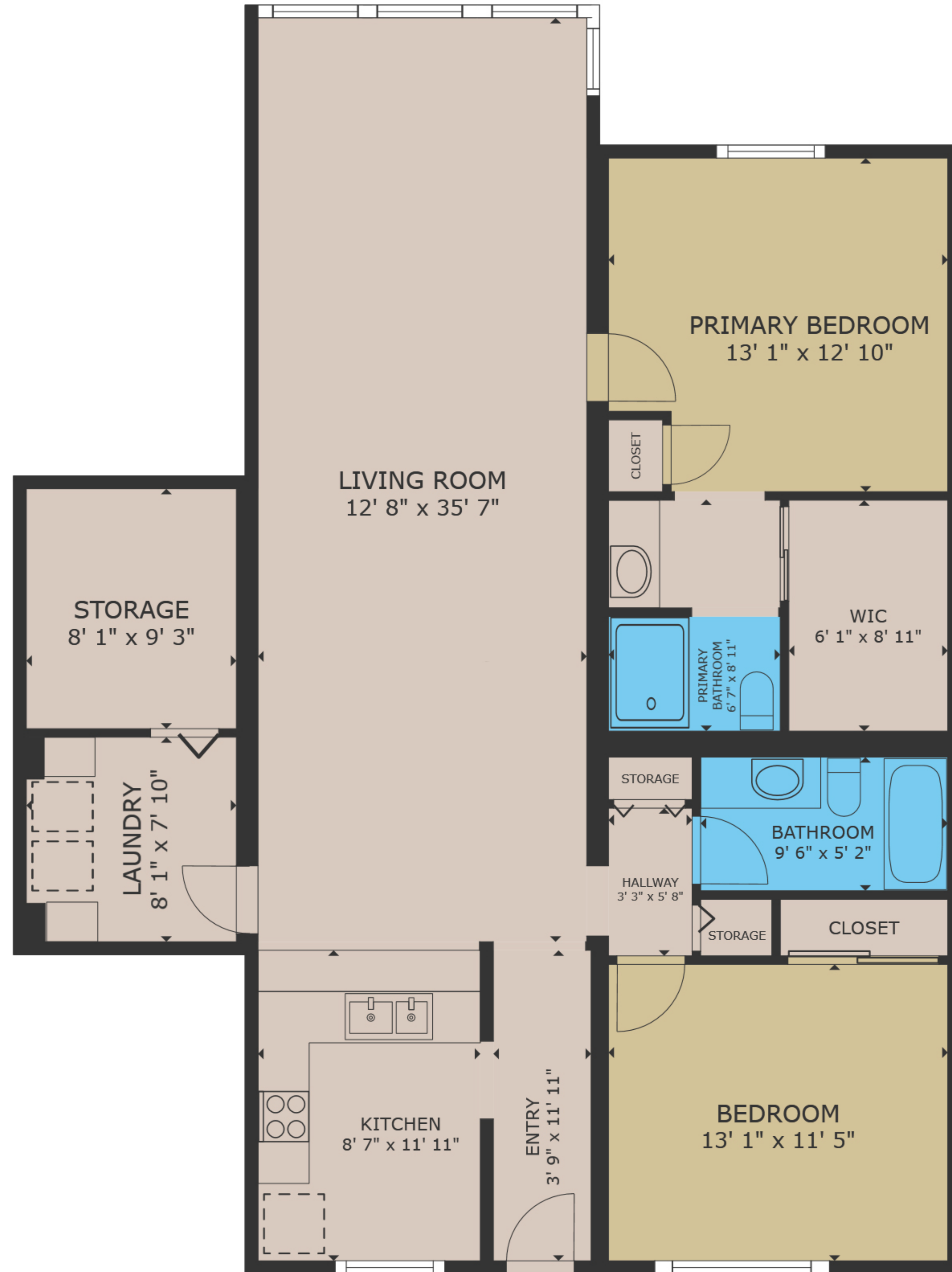
FLOOR PLAN
